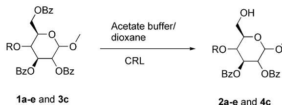
Scheme 2. CRL-catalysed hydrolysis of 1a–e and 3c . 1a–e : R = Bz, 3c : R = H.
