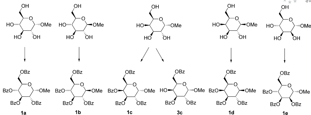
Scheme 1. Synthesis of starting materials: a : \alpha -D-glucopyranoside, b : \beta -D-glucopyranoside, c : \alpha -D-galactopyranoside, d : \beta -D-galactopyranoside, e : \alpha -D-mannopyranoside.
